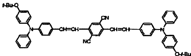
Structural formula (15)-7:
